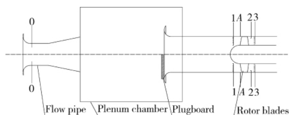
0-0 flow rate static pressure holes; 1-1 inlet total pressure combs; 2-2 Kulite dynamic pressure probes of exit; 3-3 exit total pressure combs; A-A Kulite dynamic static pressure sensors CH1 to CH4.
