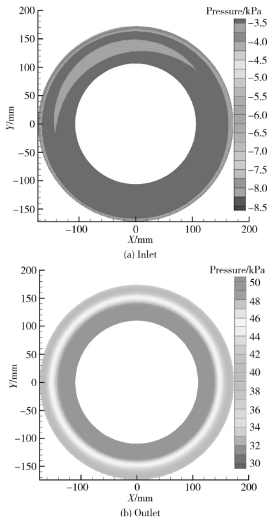
Fig. 6 Uniform inlet and outlet total pressure contours
