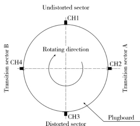
Fig. 2 Schematic of circumferential sectors in compressor
