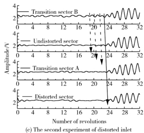
Fig. 15 Propagation of disturbances in circumferential direction
