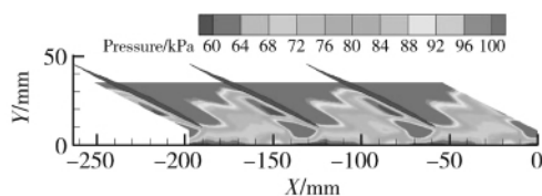
Fig. 10 Maps of casing wall static pressure of uniform inlet by experiment
